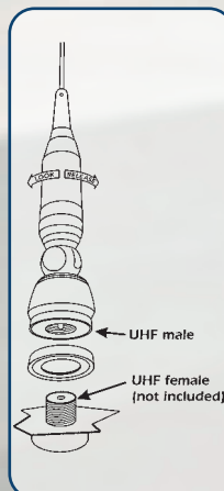
UHF-PL INSTALLATION
