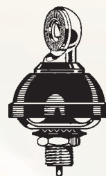
N mount black Mounting hole: \varnothing 12.5mm Overall size: \varnothing 41mm 2500102.02
